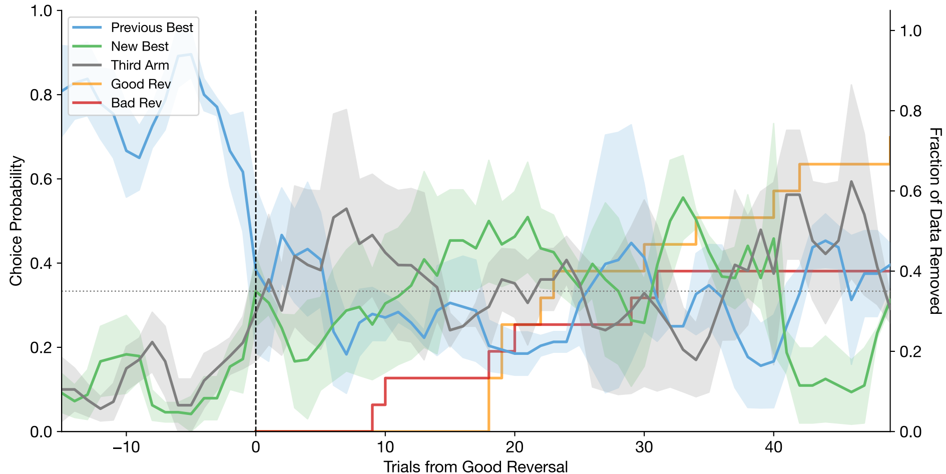
Good Reversal-Aligned Choices (mean \pm se across subjects | n=3 subjects, n=15 reversals)
